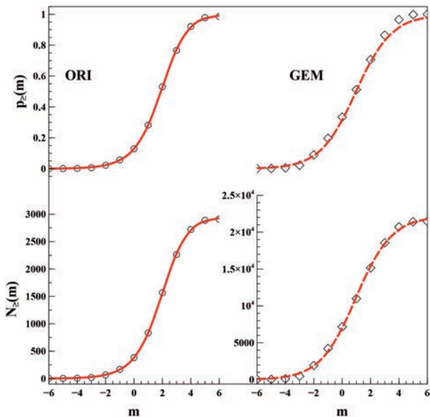
Fig. 5. Absolute ( N_{\geq}(m) ) and relative percentage ( 100\% \times N_{\geq}(m)/N_{\text{t}} ) distributions of the apparent magnitudes m of meteor showers GEM (diamonds) and ORI (circles) observed in 2012. The red lines represent the adjustments of the equation 11, with N_{\text{t}} = 22,243 , \beta_{\text{q}} = 2.07 , \gamma = 0.77 and q' = 1.94 (dashed) and N_{\text{t}} = 2,953 , \beta_{\text{q}} = 11.12 , \gamma = 1.94 , and q' = 2.34 (continuous).
