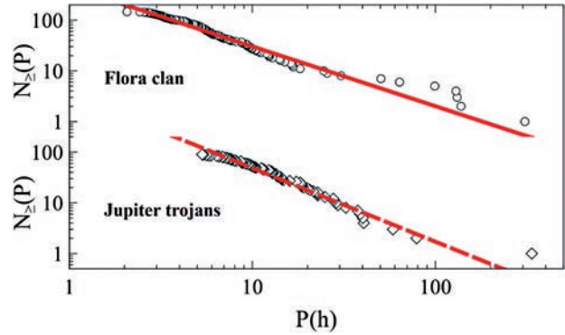
Fig. 2. Cumulative decreasing distributions of the rotation periods of 146 asteroids from the Flora clan (circles) and 90 Jupiter Trojans asteroids (diamonds). The adjustment of a power law of the type N_{\ge}(P) = aP^b is represented by the red lines: a = 455 \pm 6 , b = -1.178 \pm 0.007 (continuous), and a = (1.37 \pm 0.03) \times 10^3 , b = -1.452 \pm 0.008 (dashed). Considering b = 1/(1-q) , the values of b imply q = 1.849 \pm 0.005 and 1.689 \pm 0.004 for the asteroids of the Flora clan and the Jupiter Trojans. Data obtained from Kryszczyńska et al. (2012) and Mottola et al. (2011).
