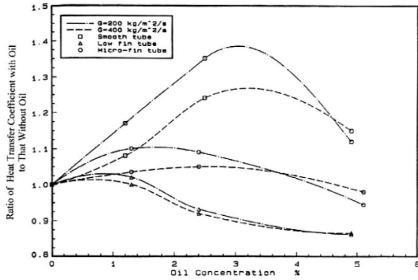
Fig. 14. Influence of oil on average evaporation heat transfer coefficients for plain and internally finned tubes (Schlager et al., 1988).
