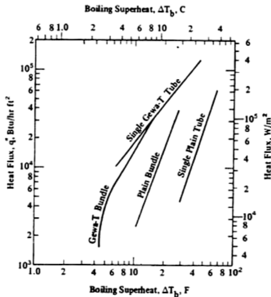
Fig. 7. Comparison of performance for single enhanced and plain tubes to that of enhanced and plain tube bundles with p-xylene at 103 kPa (Yilmaz et al., 1980).
