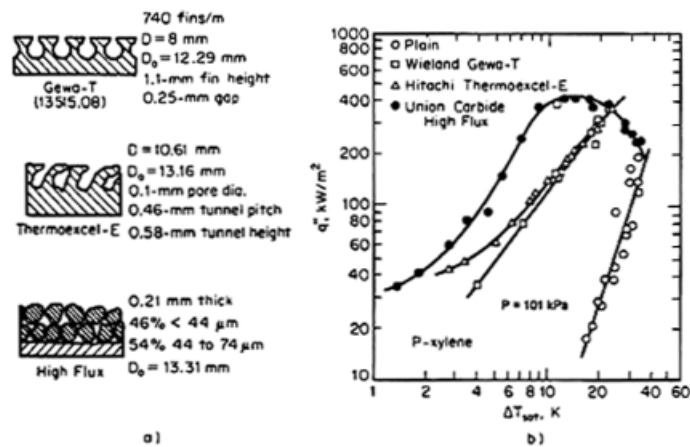
Fig. 4. Pool boiling from smooth and structured surfaces on the same apparatus (Yilmaz et al., 1980): a) Sketches of cross-sections of the three enhanced heat transfer surfaces tested; b) Boiling curves for the enhanced tubes and a smooth tube.
