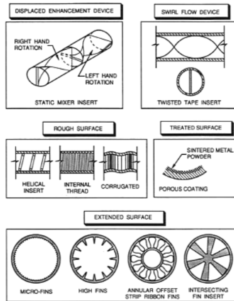
Fig. 8. Examples of passive enhancement techniques for forced-convection boiling and evaporation (Schlager et al., 1989).
