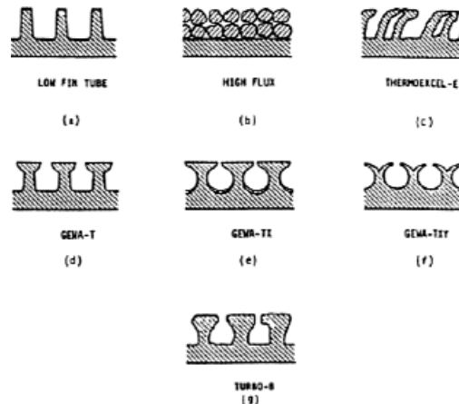
Fig. 3. Examples of structured boiling surfaces (Pate et al., 1990).
