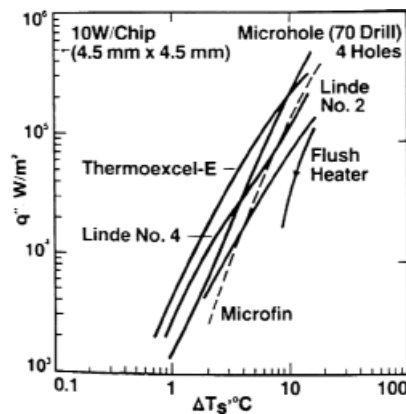
Fig. 5. Composite of data for heat sinks boiling in R-113 (Park and Bergles, 1986).
