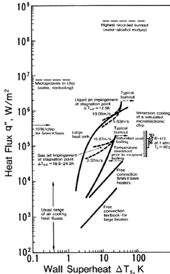
Fig. 1. Heat flux (chip level) ranges for immersion cooling of microelectronic chips; air and water capabilities are provided for reference (Bergles, 1989).
