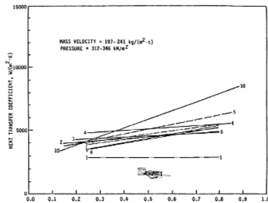
Fig. 12. Average evaporation heat transfer coefficients (R-113) for micro-fin tubes and a plain tube (Khanpara et al., 1986).
