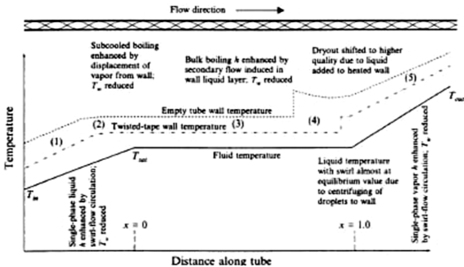
Fig. 15. The influence of twisted-tape-induced swirl on the evolution of fluid-bulk and tube-wall temperatures along the tube length in forced-convection vaporization (Manglik and Bergles, 2002).
