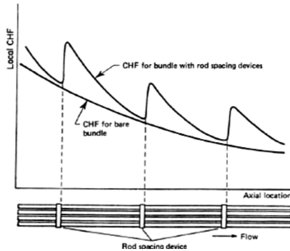
Figure 16. Effect of rod-spacing devices on CHF (Groeneveld and Yousef, 1980).
