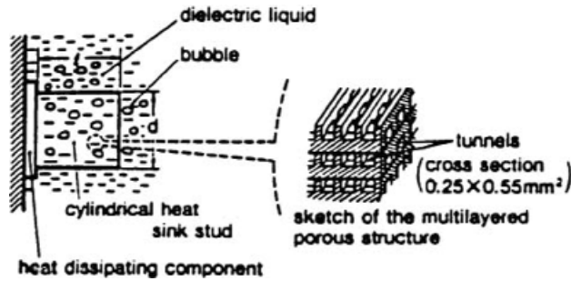
Fig. 6. Porous stud attached to the face of a heat-dissipating component (Nakayama et al., 1984).
