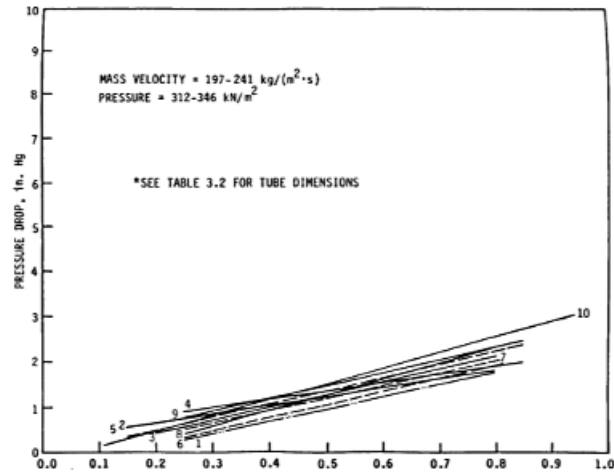
Fig. 13. Evaporation pressure drops (R-113) for micro-fin tubes and a plain tube (Khanpara et al., 1986).
