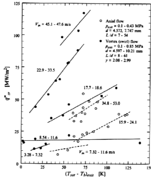
Fig. 9. Influence of twisted-tape-generated swirl flow on subcooled-boiling critical heat flux with water (Gambill et al., 1961).
