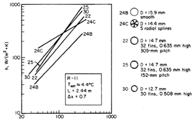
Fig. 10. Average heat transfer coefficients for evaporation in internally finned tubes (Kubanek and Miletta, 1979).
